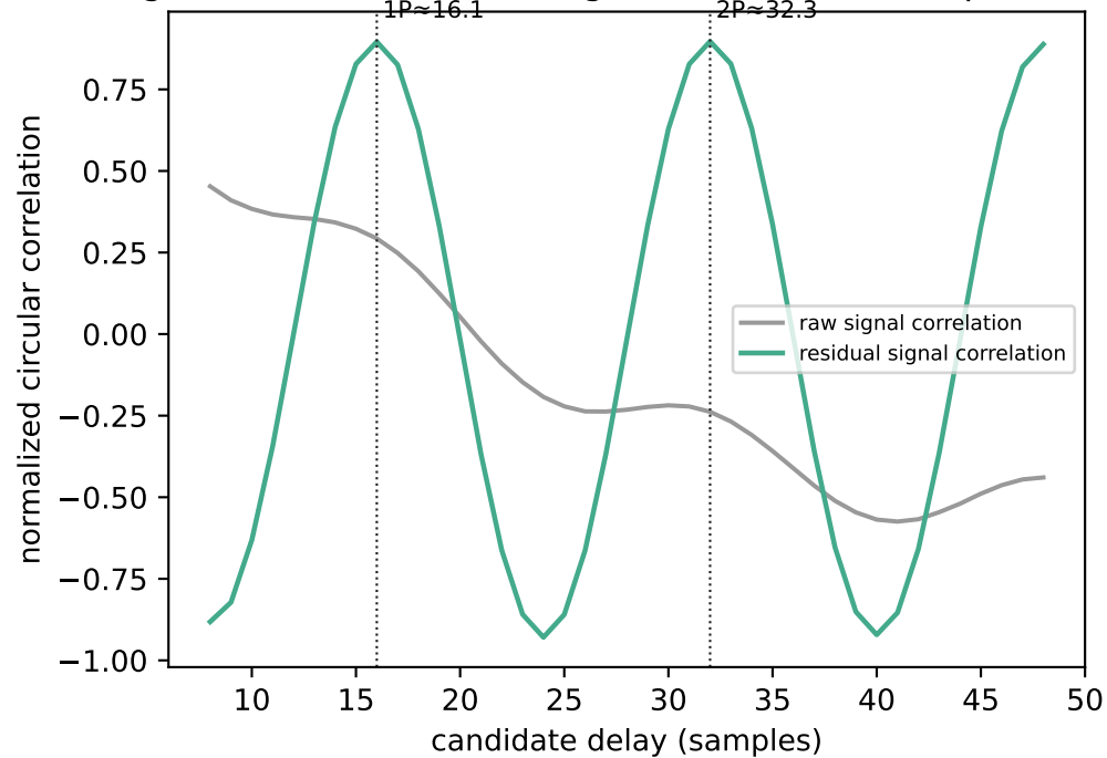
Signal-level recurrence diagnostic (not learned q/k scores)
